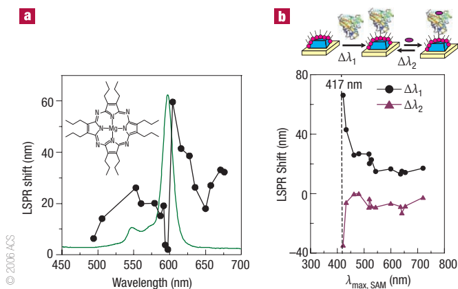
Figure 4 Wavelength-dependent LSPR shifts induced by resonant molecules. a , Comparison of LSPR shifts induced by a monolayer of MgPz adsorption on silver nanoparticles with the LSPR of bare silver nanoparticles (black line with dots). Inset: molecular structure of MgPz. Reprinted with permission from ref. 70. The green line is the solution absorption spectrum of MgPz. b , Schematic representation of CYP101 immobilized on a silver nanobiosensor followed by binding of camphor, and plots of LSPR shifts against \lambda_{\max,\text{SAM}} (LSPR of SAM-functionalized nanoparticles), where \Delta\lambda_1 is the shift on binding of CYP101 and \Delta\lambda_2 is the shift on binding of camphor. The vertical black dotted line denotes the molecular resonance of substrate-free CYP101. Reprinted with permission from ref. 72.
