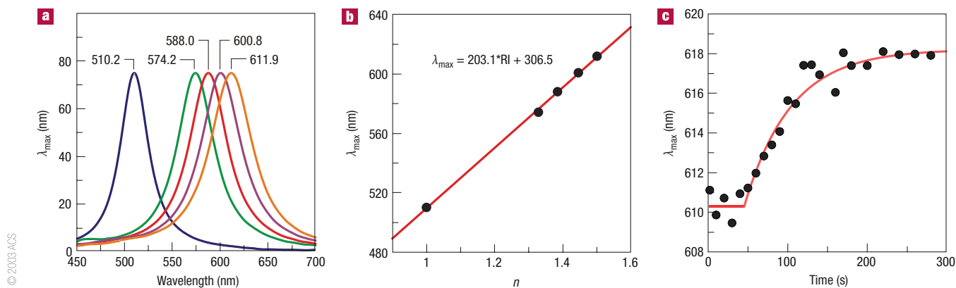
Figure 2 Single-nanoprisim LSPR. a , Resonant Rayleigh scattering spectrum from a single silver nanoparticle in various solvent environments (left to right): nitrogen, methanol, propan-1-ol, chloroform and benzene. b , Plot depicting the linear relationship between the solvent refractive index n and the LSPR \lambda_{\max} ; the regression equation is \lambda = 203.1n + 306.5 . c , Monitoring the real-time adsorption of octanethiol (1 mM) onto a single nanoparticle. At this concentration, the rate constant is estimated to be 0.017 \text{ s}^{-1} . Reprinted with permission from ref. 11.
